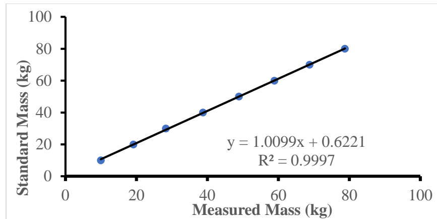
Figure 6: Calibration Curve of the Load Cell
