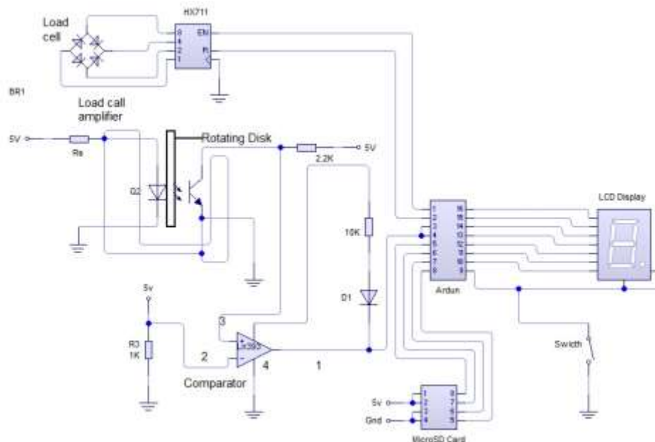
Figure 4. Circuit Diagram for the Instrumentation System
